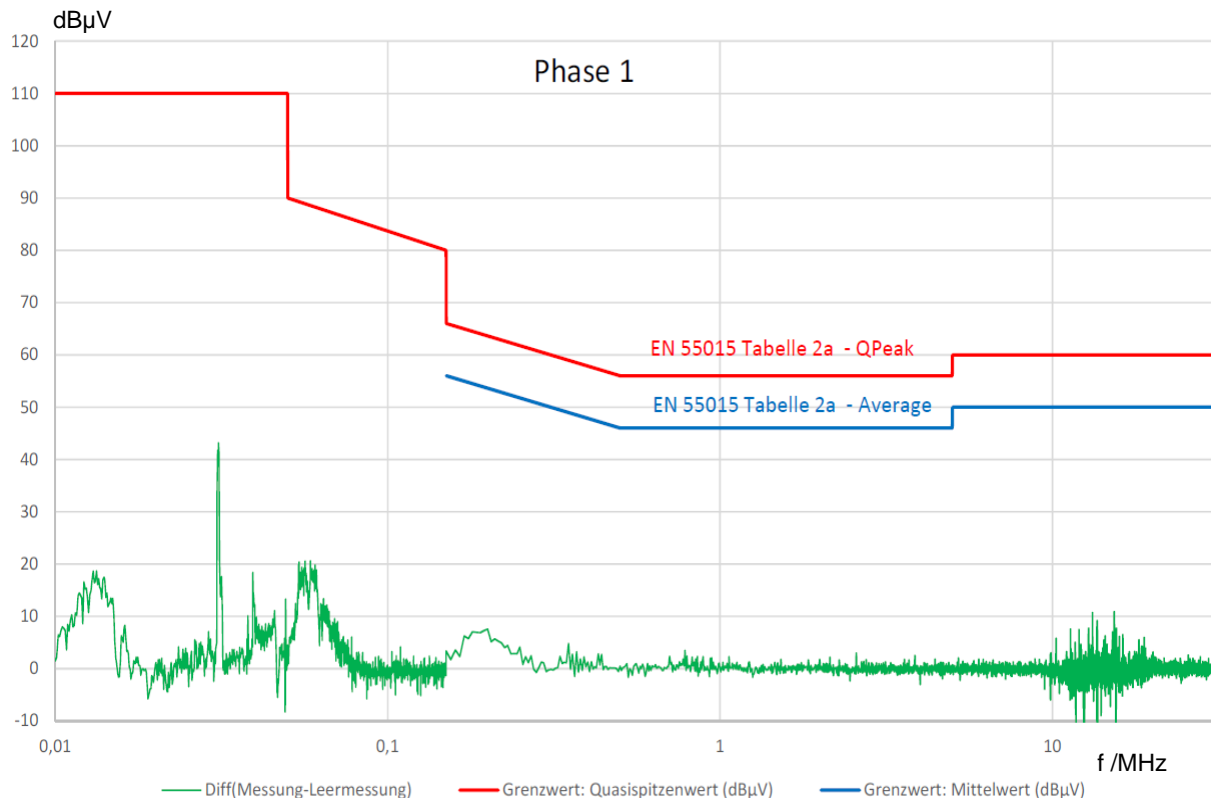
Figure 2: Example of interference voltage at full load according to EN 55015 and EN 61547
